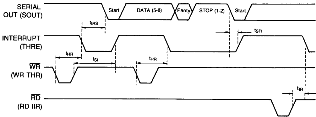
Transmitter Timing
