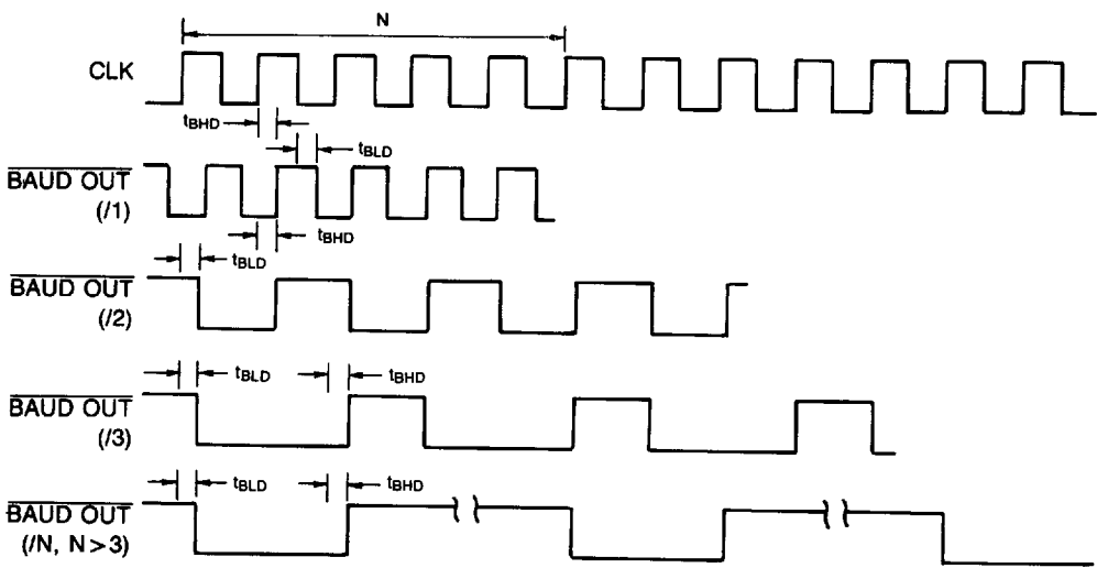
Baudout Timing
